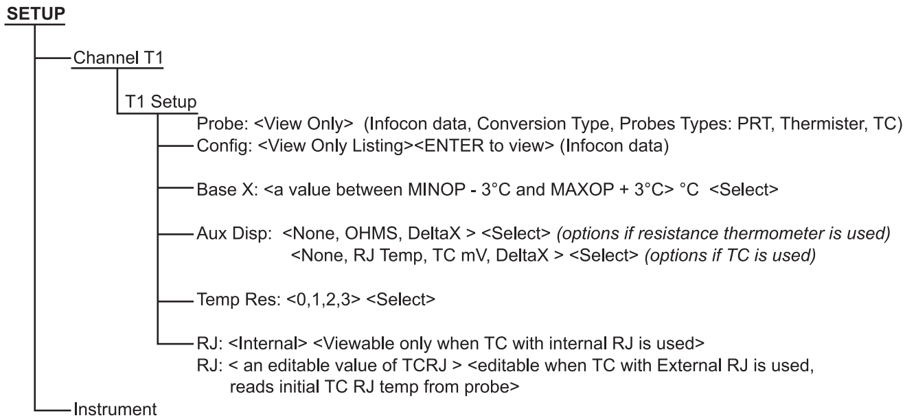
Figure 6 1523 Menu
