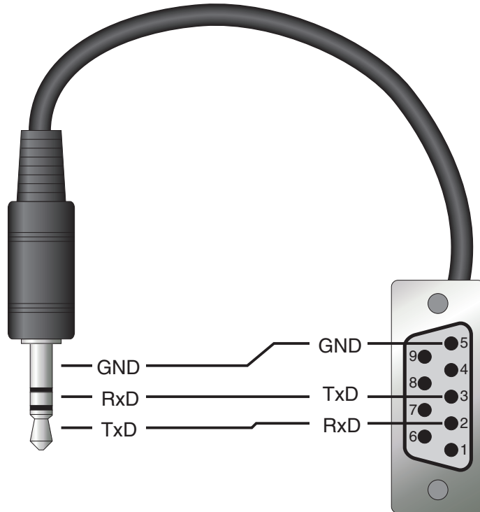
Figure 17 RS-232 wiring
